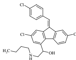
Molecular Weight =472.85 Molecular Formula =C26H24Cl3NO
