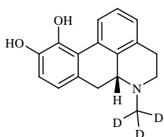
Molecular Weight =270.35 Molecular Formula =C17H14NO2D3
