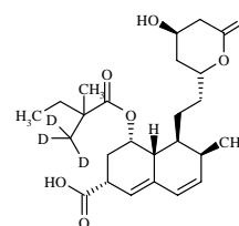
Molecular Weight =451.58 Molecular Formula =C25H33O7D3
