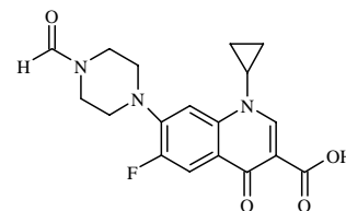
Molecular Weight =359.36 Molecular Formula =C18H18FN3O4
