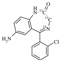
Molecular Weight =288.71 Molecular Formula =C15H12ClN3O
