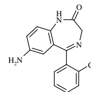
Molecular Weight =285.74 Molecular Formula =C15H12ClN3O
