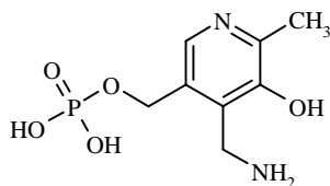
Molecular Weight =248.18 Molecular Formula =C8H13N2O5P
