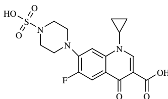
Molecular Weight =411.41 Molecular Formula =C17H18FN3O6S
