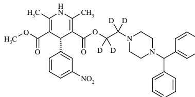
(R)-(-)-Manidipine-d 4
