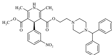
(S)-(+)-Manidipine
