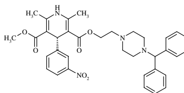
(R)-(-)-Manidipine
