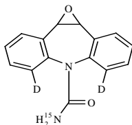
Carbamazepine-d 2 - 15 N 1 -10,11 epoxide
