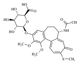
3-Desmethylthiocolchicine-3-Glucuronide
