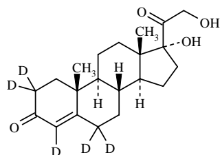
Molecular Weight =351.50 Molecular Formula =C 21 H 25 O 4 D 5
