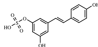
Molecular Weight =308.31 Molecular Formula =C 14 H 12 O 6 S
