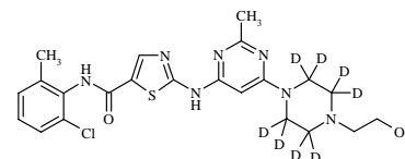
Molecular Weight =496.06 Molecular Formula =C 22 H 18 ClN 7 O 2 S 2 D 8
