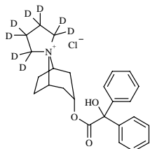
Molecular Weight =400.57 35.45 Molecular Formula =C 25 H 22 NO 3 D 8 . Cl
