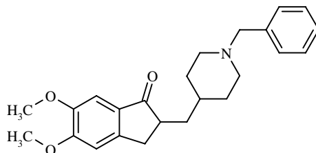
Molecular Weight =379.50 Molecular Formula =C 24 H 29 NO 3 (-)-Donepezil
