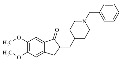
Molecular Weight =379.50 Molecular Formula =C 24 H 29 NO 3 (+)-Donepezil
