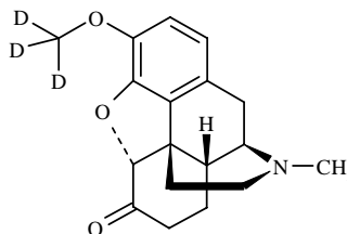
Molecular Weight =302.39 Molecular Formula =C 18 H 18 NO 3 D 3
