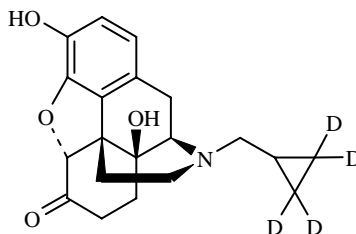
Desmethyl Butenafine
