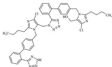
Dimeric degradate of Losartan (Known as Isomer E)
