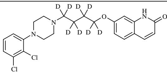
Aripiprazole-dehydro-d8
