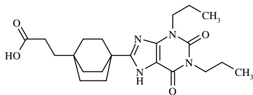
4-(2,3,6,7-tetrahydro-2,6-dioxo-1,3-dipropyl-1H-purin-8-yl)-Bicyclo[2.2.2]octane-1-propanoic acid
