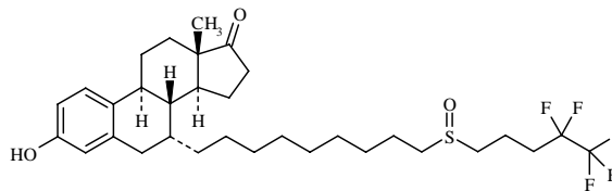
Fulvestrant 17-ketone
