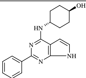
trans-4-[(2-phenyl-7H-pyrrolo[2,3-d]pyrimidin-4-yl)amino]-Cyclohexanol
