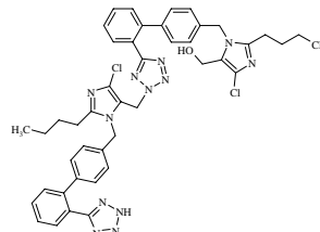
Dimeric degradate of Losartan (Known as Isomer F)
