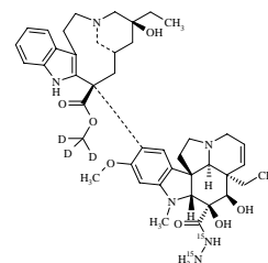
Molecular Weight =773.97 Molecular Formula =C 43 H 53 N 6 O 7 D 3
