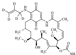
Molecular Weight =590.73 Molecular Formula =C 31 H 38 N 3 O 8 D 5
