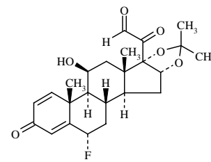
Molecular Weight =432.49 Molecular Formula =C 24 H 29 F 2 O 6
