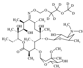
Molecular Weight =844.11 Molecular Formula =C 41 H 69 N 2 O 15 D 7
