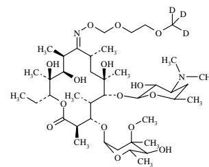
Molecular Weight =840.09 Molecular Formula =C 41 H 73 N 2 O 15 D 3
