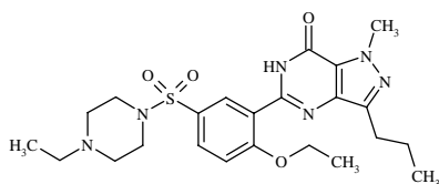
Molecular Weight =488.61 Molecular Formula =C 23 H 32 N 6 O 4 S
