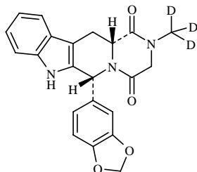
Molecular Weight =392.43 Molecular Formula =C 22 H 16 N 3 O 4 D 3
