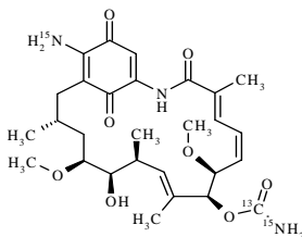
Molecular Weight =548.61 Molecular Formula =C 28 H 39 N 3 O 8
