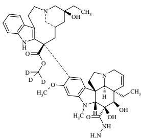
Desacetylvinblastine-d 3 hydrazide
